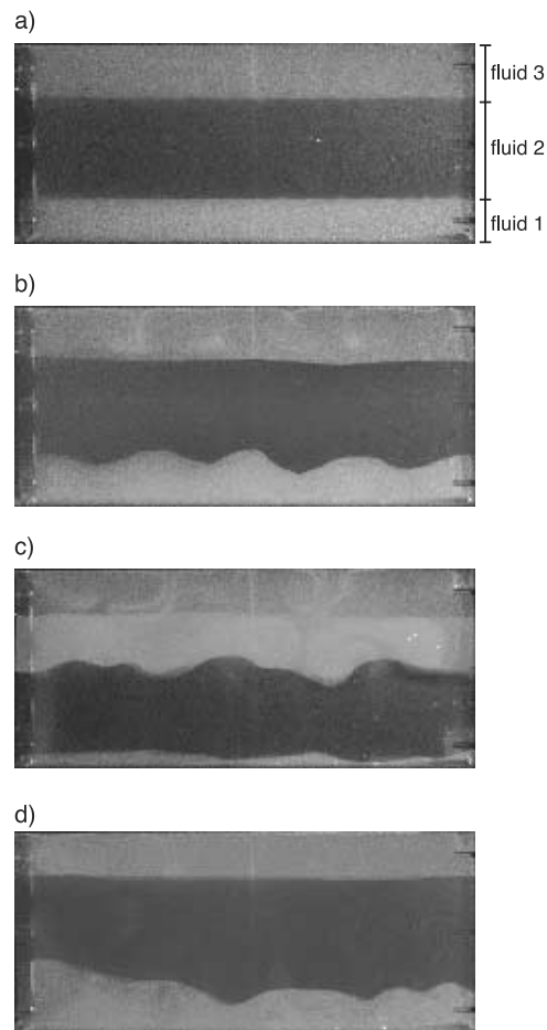
Figure 18. Experiment with three layers ( h_1 = 3.0 cm, h_2 = 7.8 cm, h_3 = 4.0 cm, \gamma_{1-2} = 56 , \gamma_{2-3} = 3.6 , B_{1-2} = 0.24 , B_{2-3} = 1.46 , Ra = 4.4 \times 10^7 ): (a) t = 0 min, (b) t = 12 min, (c) t = 17 min, and (d) t = 24 min. See color version of this figure in the HTML.
