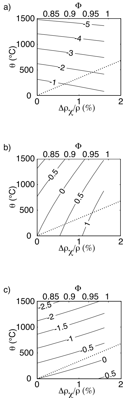
Figure 15. Predicted seismic anomaly in percent depending on the local temperature excess \theta and the chemical density contrast \Delta\rho_\chi/\rho , taking x_{\text{Fe}} = 0.11 in both layers, \Phi = 0.82 in the upper layer and a variable \Phi in the lower layer (top scale): (a) shear waves, (b) bulk sound, and (c) compressional waves. Dotted lines show the “equilibrium” position, where thermal effects compensate for chemical stratification as given by the mean equation (14).
