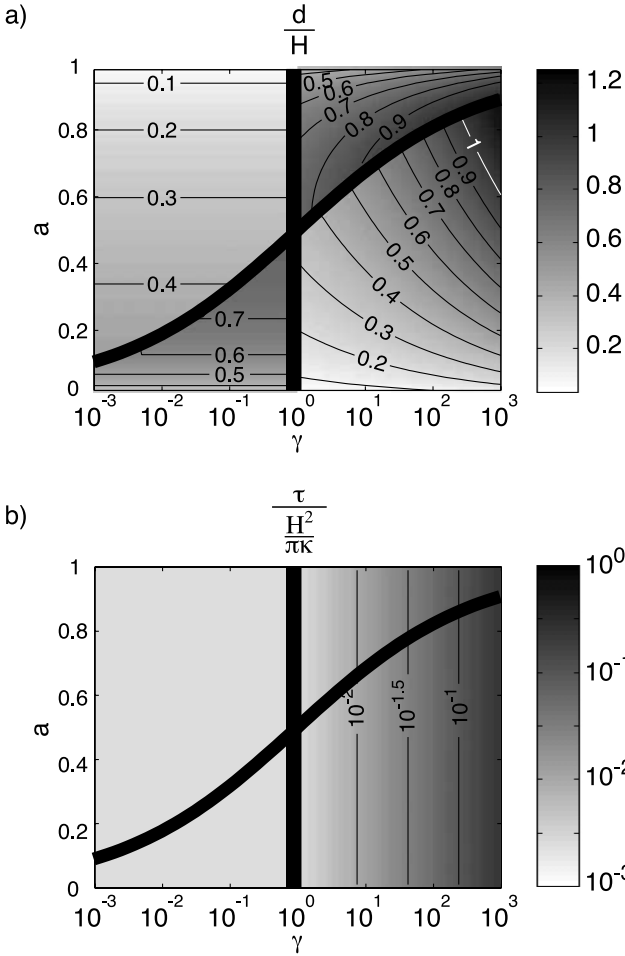
Figure 9. (a) Nondimensional diameter and (b) nondimensional period of thermochemical structures in planetary mantle as a function of the viscosity ratio \gamma and the layer depth ratio a , taking a Rayleigh number Ra = 1.3 \times 10^7 . Thick black lines indicate changes in the shape of thermochemical domes, as explained in section 2.1 and in Figure 3.
