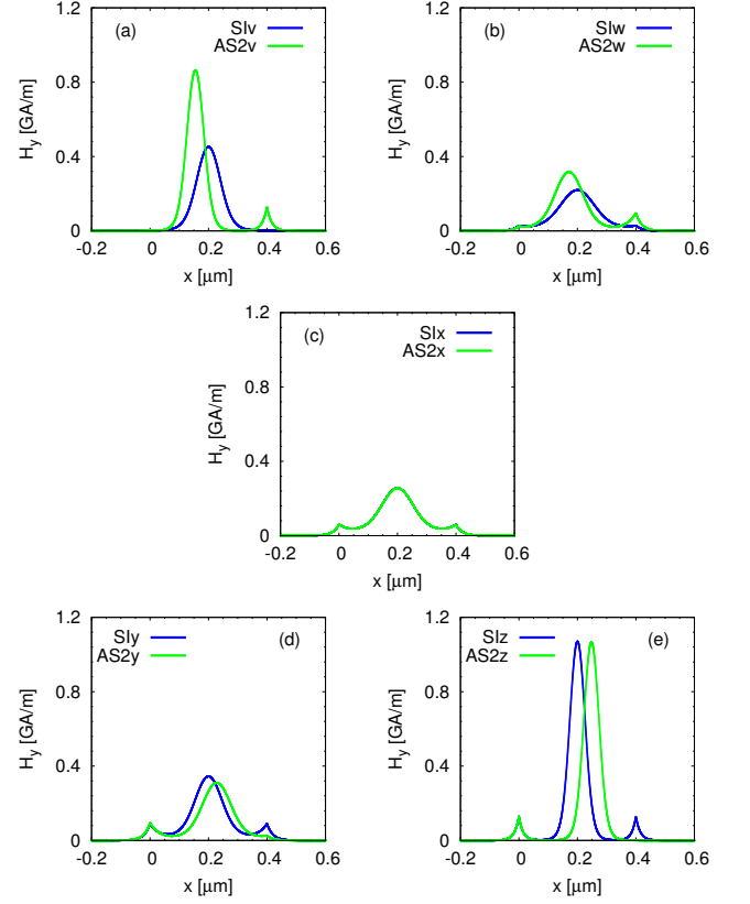
FIG. 4. Profiles of magnetic field H_y(x) for the symmetric SI mode (blue) and the second-order asymmetric AS2 mode (green). The subplots present the transformation of the field profiles at the points corresponding to the vertical lines labeled v-z indicated in Fig. 6. In each subplot the value of E_0 {see Eq. ([equation][28][28] in Ref. [18] for its definition} is identical for both modes.
