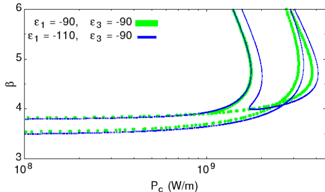
FIG. 13. Dispersion curves of the asymmetric NSW with \epsilon_1 = -110, \epsilon_3 = -90 (blue curves) and the symmetric structure \epsilon_1 = \epsilon_3 = -90 (green curves).
