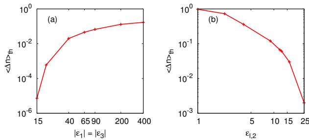
FIG. 10. Average nonlinear index change at the appearance of the asymmetric AS1 modes \langle \Delta n \rangle_{th} as a function of the absolute value of (a) the metal cladding permittivity of the symmetric waveguide |\epsilon_1| = |\epsilon_3| and (b) the linear part of the nonlinear core permittivity \epsilon_{l,2} . All the other parameters of the NSW are identical to these used in Sec. II A.
