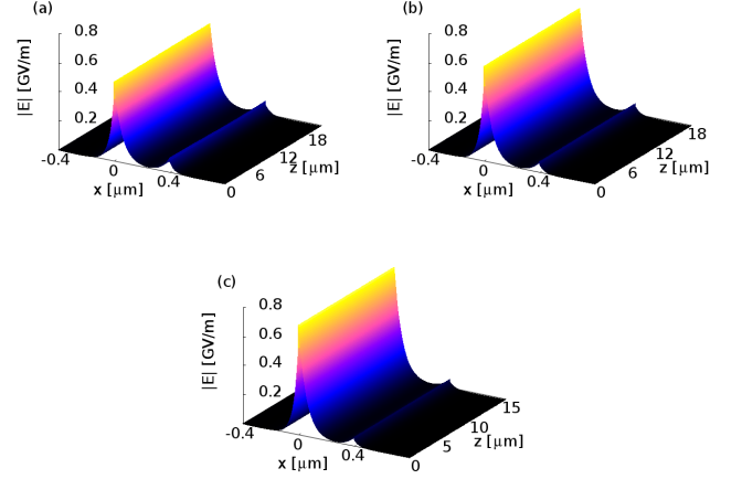
FIG. 23. Evolution of the electric field norm during the propagation of asymmetric modes located between the Hopf bifurcation and the fold bifurcation. The average nonlinear index change in the core ( \langle \Delta n \rangle ) induced by these modes is equal to (a) 2 \cdot 10^{-3} , (b) 3 \cdot 10^{-3} , and (c) 4 \cdot 10^{-3} . The shown propagation distance is approximately 12 free-space wavelengths. The parameters are the same as in Fig. 22. These simulations are realized using the COMSOL software.
