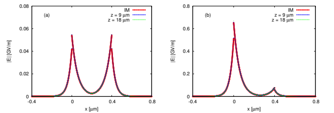
FIG. 25. Comparison of the |E| profiles obtained using the IM (and used as the input profiles in the COMSOL based simulations) and cuts of the field evolution in the middle of the propagation range ( z = 9 \mu\text{m} — 6 free-space wavelengths) and at the end of the propagation ( z = 18 \mu\text{m} — 12 free-space wavelengths) for (a) the symmetric nonlinear plasmon-soliton (see Fig. 22) and (b) the asymmetric nonlinear plasmon-soliton [see Fig. 23(b)].
