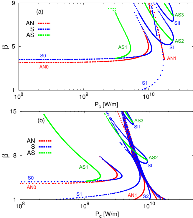
FIG. 1. Dispersion diagrams \beta(P_c) for the symmetric NSW obtained using (a) the JEM and (b) the IM.
