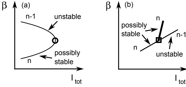
FIG. 15. Rules of assigning the stability of the modes for two specific cases extracted from Fig. 2 in Ref. [23]: (a) the fold bifurcation (open circle) and (b) the Hopf bifurcation (open square). Thick lines indicate a doubly degenerate branch, whereas thin lines indicate non-degenerate dispersion curves.
