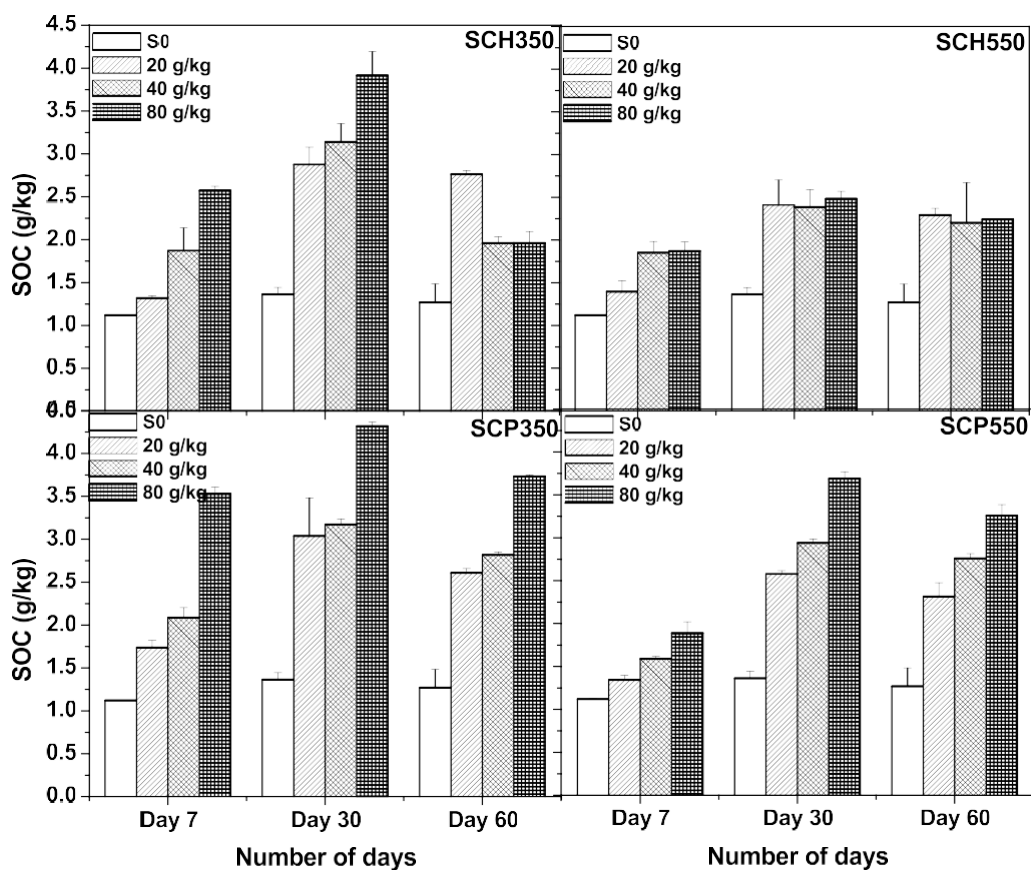
Figure 5. Effect of biochar application rate and incubation time on acidic soil with soil organic carbon.
