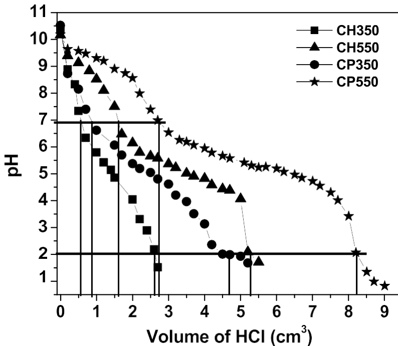
Figure 1. Acid-base titration curves of biochars produced from coffee husk and cocoa pods at different pyrolysis temperatures.
