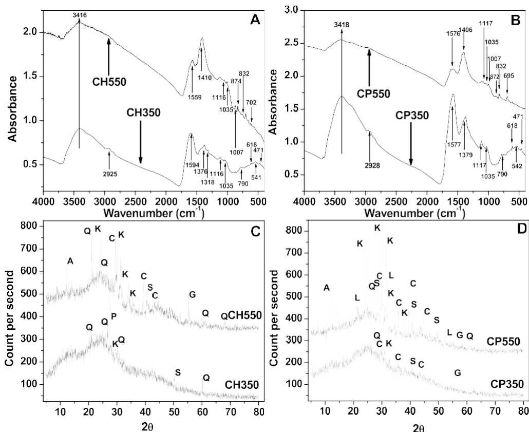
Figure 2. FTIR analysis of (A) CH350 and CH550, (B) CP350 and CP550, XRD spectrum of (C) CH350 and CH550 and (D) CP350 and CP550.
