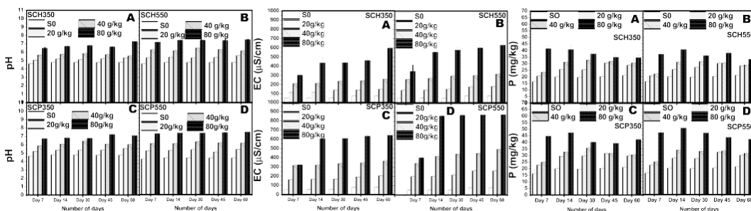
Figure 3. Effect of biochar application rate and incubation time on acidic soil with respond on soil pH (left), electrical conductivity (middle) and available P (right).
