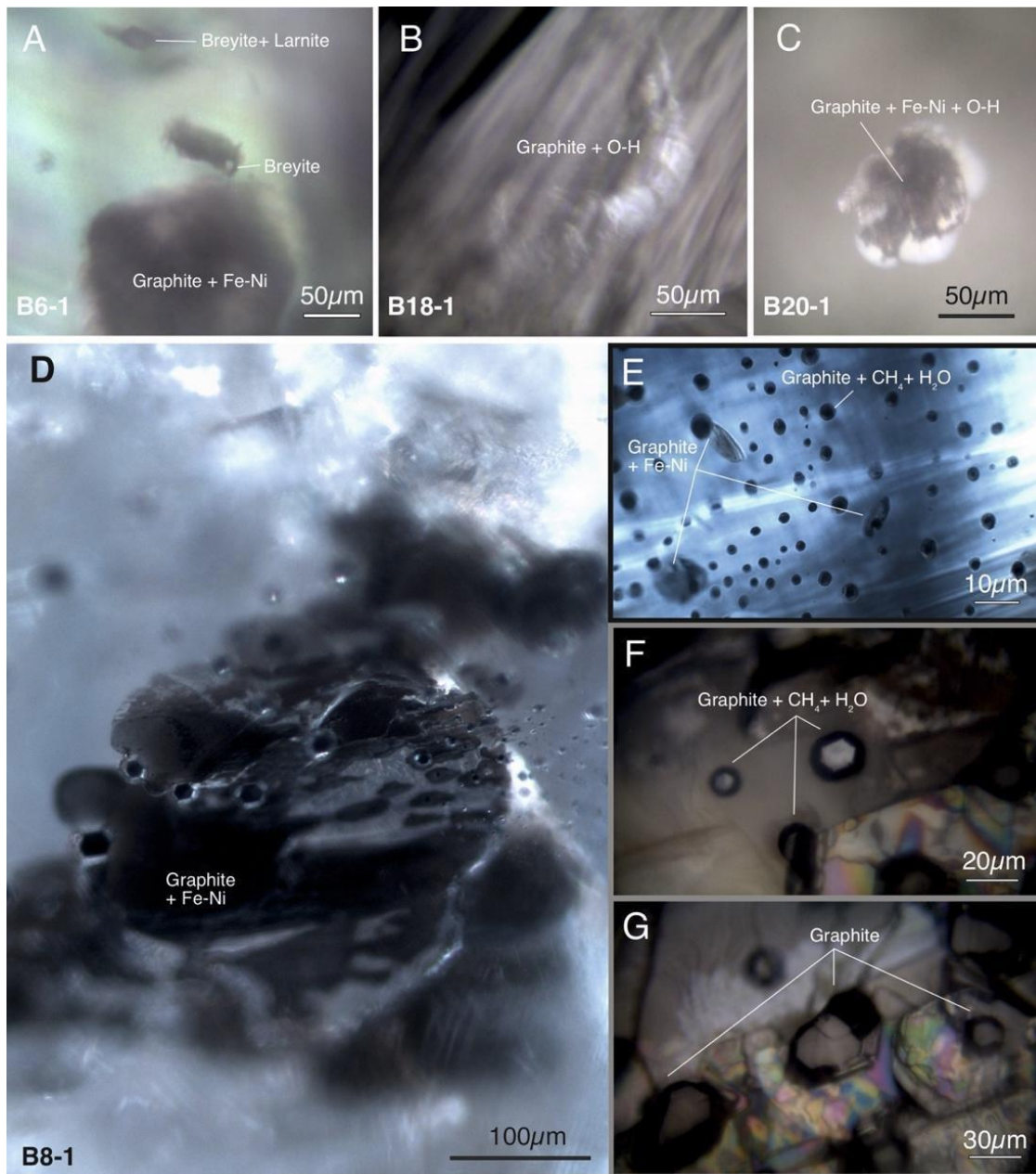
Figure 5. Images of inclusions in the studied diamonds. A) flat primary Fe-Ni-C inclusions in the center, small isolated breyite inclusions located at the bottom left and larnite and breyite inclusions at the top in sample B6-1. B) Primary graphite inclusion, surrounded by a fluid envelope in sample B18-1. C) Primary Fe-Ni and graphite inclusion, surrounded by a fluid envelope in sample B20-1. D) Secondary metallic cluster (Fe-Ni alloys and graphite) in a healed fracture in sample B8-1; small inclusions in front of the cluster are isolated graphite crystals surrounded by a fluid envelope. E) Larger view of the innermost part of the healed fracture in sample B8-1, which exhibits graphite crystals in the center, surrounded by a fluid envelope composed of water and methane (5-15 \mu\text{m} in
