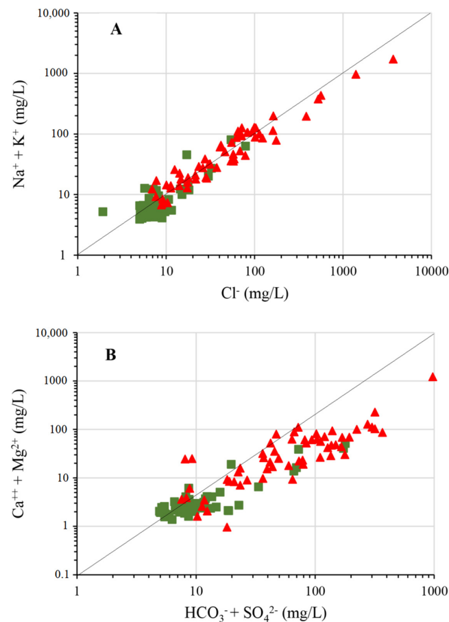
Figure 9. Bivariate plots of ionic relation. (A) \text{Na}^+ + \text{K}^+ versus \text{Cl}^- . (B) \text{Ca}^{2+} + \text{Mg}^{2+} versus \text{HCO}_3^- + \text{SO}_4^{2-} for coastal aquifers in Benin. The bisector represents the 1:1 dissolution line.
