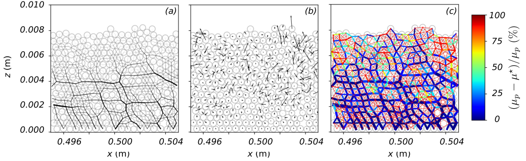
Figure 12: (a) Snapshots of the contact force chains, (b) vibration-induced displacements, and (c) rate of vibration-induced perturbation of the interparticle friction, for \theta = 15^\circ , H/d = 14.4 , f = 30 kHz, at t = 0.072 s. (a) The black lines represent the force chains formed between the grains on a linear scale (the coefficients f_n^{ij} in Section 2.2.2). (b) The black arrows represent the computed vibrational displacement \mathbf{q} in Eqs. (2.10)-(2.11). (c) The lines between grains represent the force chains on a logarithmic scale, and the color map represent the rate of decrease in interparticle friction coefficients, i.e., the quantity (\mu_p - \mu_p^*)/\mu_p (see Eq. (2.12)). The basal vibration amplitude is the same as in Fig. 10, about U_0/d = 10^{-5} .
